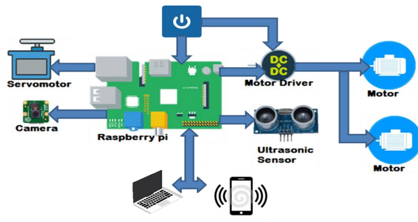
FIGURE 1: System schematic layout.
