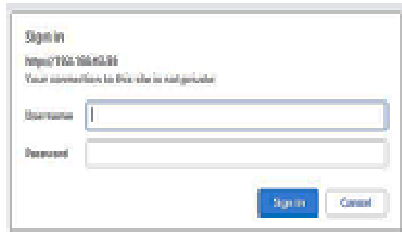
FIGURE 4: Authentication Page.
