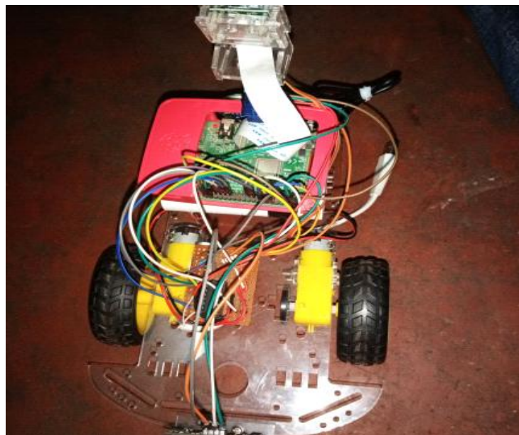
FIGURE 2: Pi-3 Robot.
